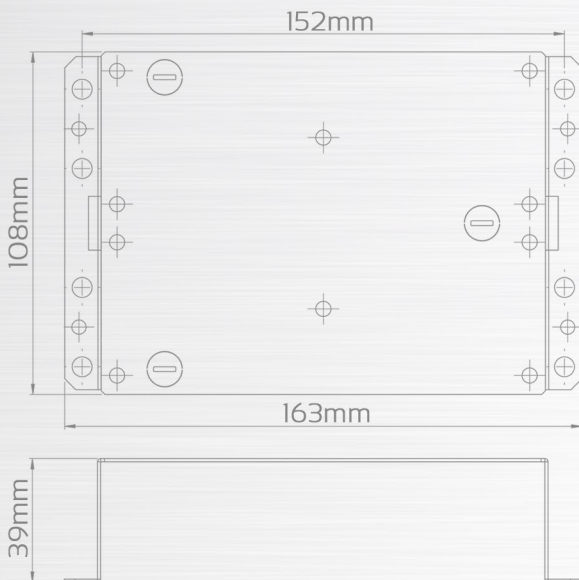
EC-SCC PLATE - Mounting Plate
