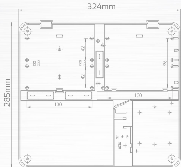
EC-CAB - Security Enclosure
